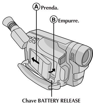
Chave BATTERY RELEASE
